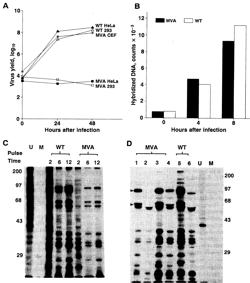
FIG. 1. Characterization of the infection of human cells with MVA. (A) Multiplication of MVA in HeLa (■), 293 (□), and CEF (*) cells and of WT in HeLa (▲) and 293 (△) cells. (B) Viral DNA synthesis was determined by hybridization of a ^{32}\text{P} -labeled viral DNA probe to DNA isolated from 293 cells at 0, 4, or 8 h after infection with MVA or WT. Radioactivity was quantitated using a Betascope 603 blot analyzer. (C) Synthesis of early and late viral polypeptides in human cells. HeLa cells were infected with WT or MVA and labeled with ^{35}\text{S} methionine at the indicated hours postinfection (Pulse Time). Cell lysates were treated with 2% SDS and 1% dithiothreitol and analyzed by electrophoresis on a 10% polyacrylamide gel. Lane U, uninfected cell extract; lane M, protein standards (indicated by their molecular masses in kDa on the left). (D) Proteolytic processing of viral proteins. CEF (lanes 1 and 2) or HeLa (lanes 3–6) cells were infected with MVA or with WT for 6 h and labeled with ^{35}\text{S} methionine for 30 min. Cells were harvested after the pulse (lanes 1, 3, and 5) or after a 16-h chase (lanes 2, 4, and 6). Cell lysates were treated with 2% SDS and 1% dithiothreitol and analyzed by electrophoresis on a 10% polyacrylamide gel. Lanes U and M are defined as in C, and the positions of the marker proteins (in kDa) are indicated on the right. The uncleaved precursors of the major late core polypeptides, P4a and P4b, are marked by arrowheads.
